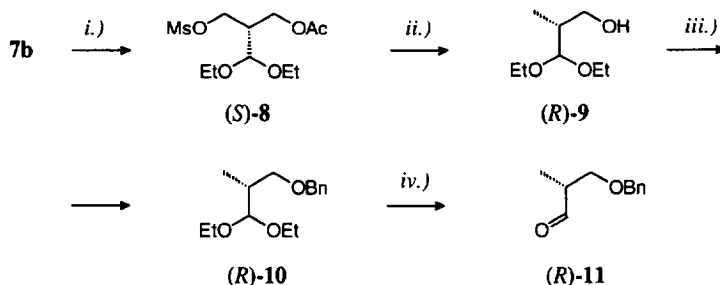
Scheme 2. Determination of the absolute configuration of the optically active monoacetate 7b . Reagents: i. ) MsCl, Et 3 N; ii. ) LiAlH 4 ; iii. ) BnCl, NaH; iv. ) cat. HCl, AcOH-H 2 O.
